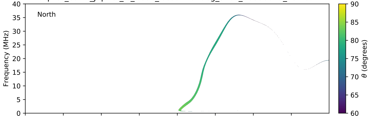
expres_earth_jupiter_io_isaac_lossc-wid1deg_3kev_20080623_v01.cdf
