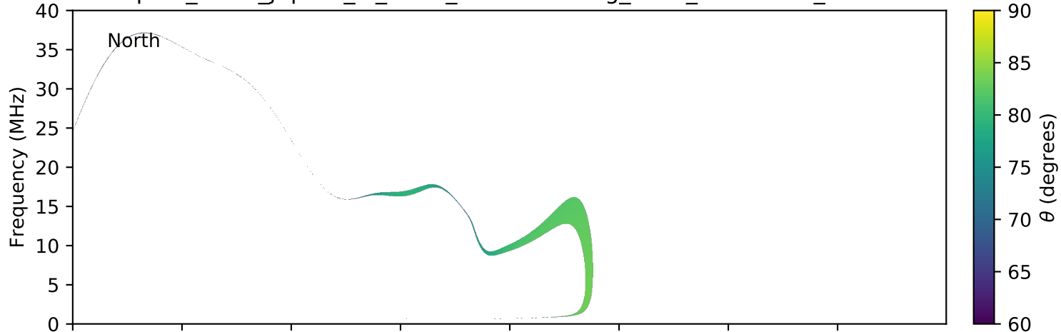
expres_earth_jupiter_io_isaac_lossc-wid1deg_3kev_20080622_v01.cdf
