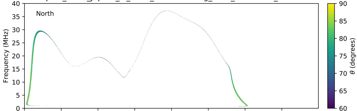
expres_earth_jupiter_io_isaac_lossc-wid1deg_3kev_20080620_v01.cdf
