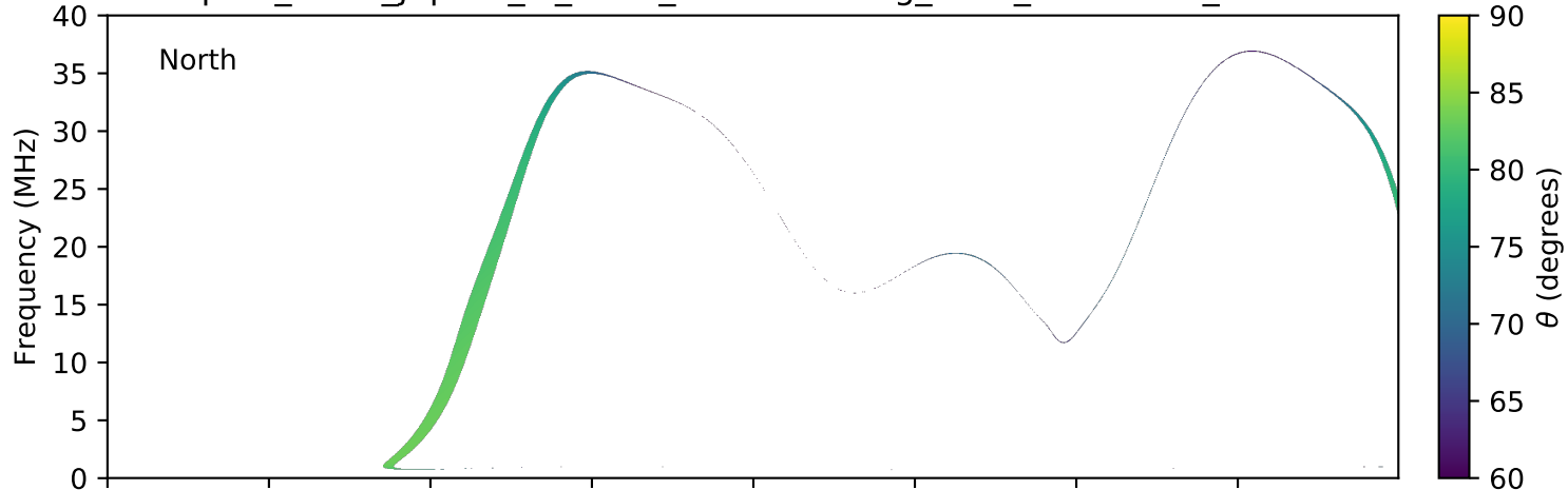
expres_earth_jupiter_io_isaac_lossc-wid1deg_3kev_20080618_v01.cdf
