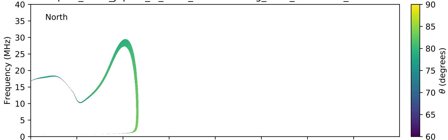
expres_earth_jupiter_io_isaac_lossc-wid1deg_3kev_20080617_v01.cdf
