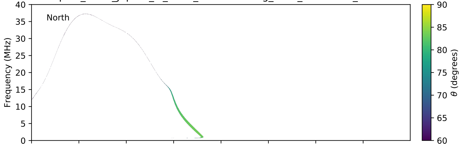
expres_earth_jupiter_io_isaac_lossc-wid1deg_3kev_20080615_v01.cdf
