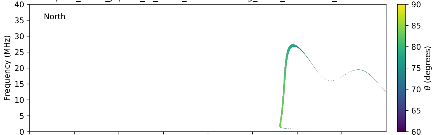
expres_earth_jupiter_io_isaac_lossc-wid1deg_3kev_20080614_v01.cdf
