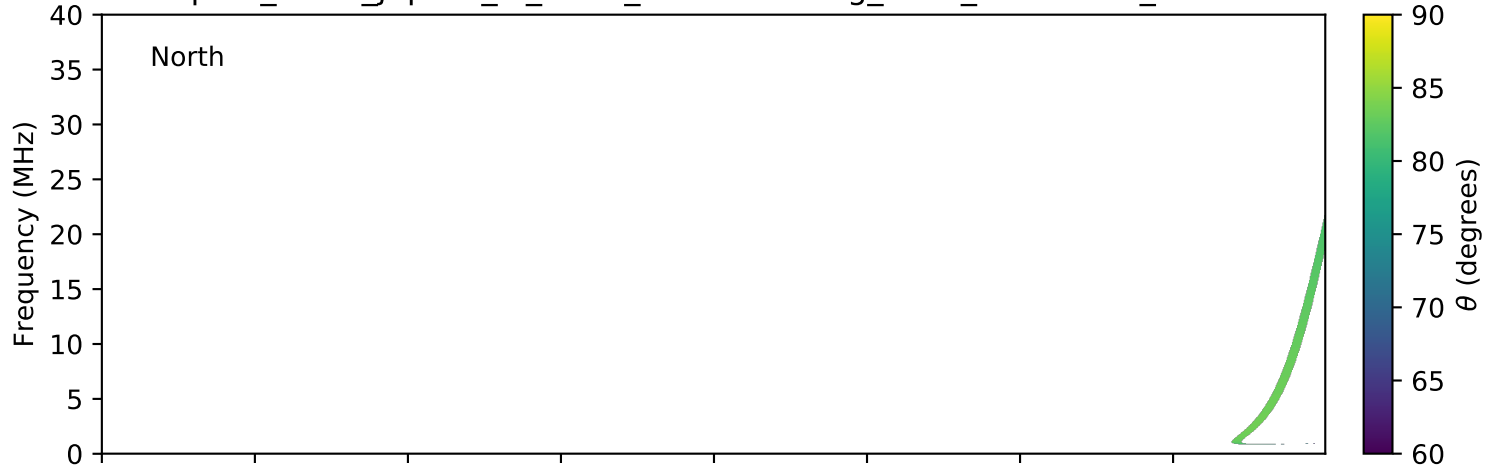
expres_earth_jupiter_io_isaac_lossc-wid1deg_3kev_20080612_v01.cdf
