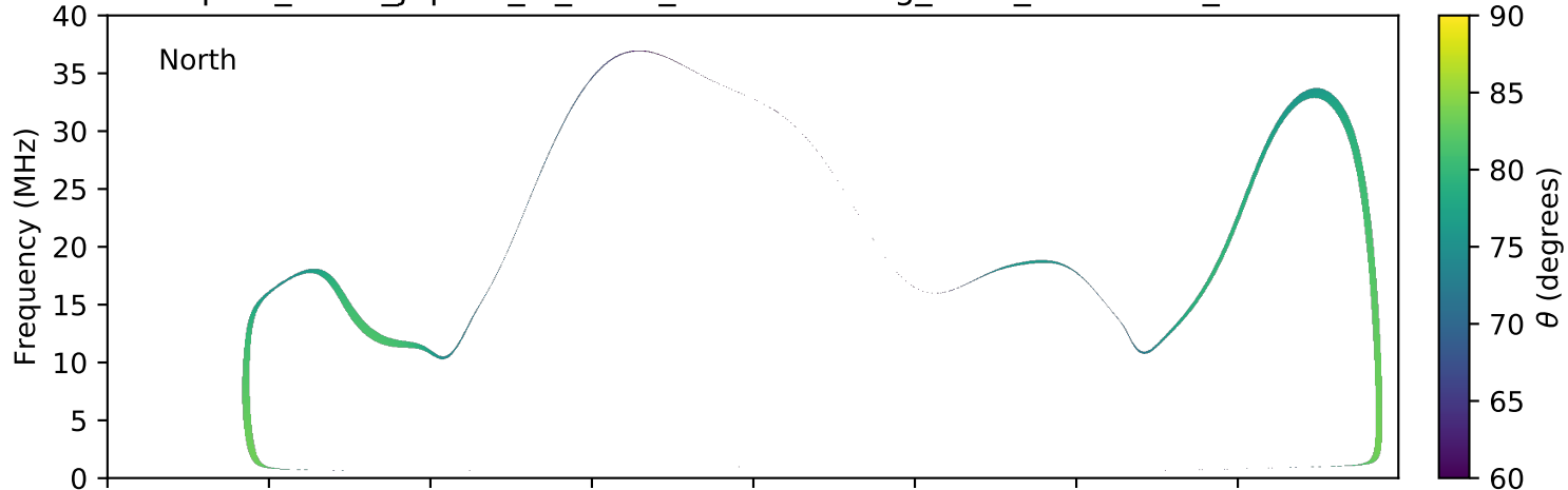
expres_earth_jupiter_io_isaac_lossc-wid1deg_3kev_20080611_v01.cdf
