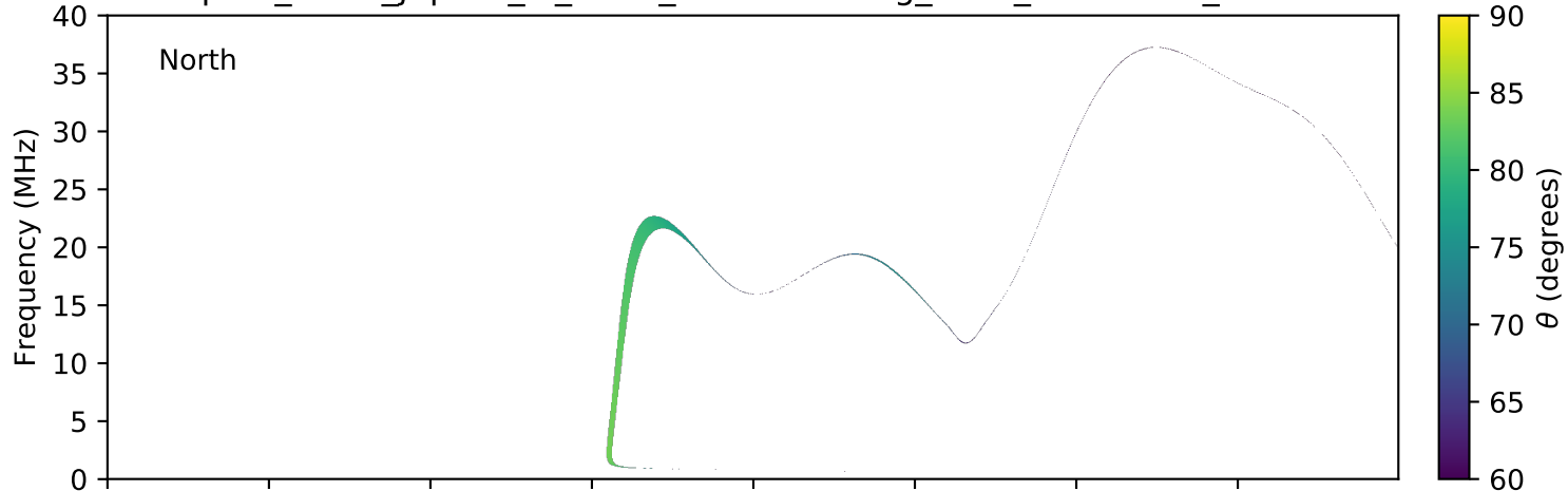
expres_earth_jupiter_io_isaac_lossc-wid1deg_3kev_20080609_v01.cdf
