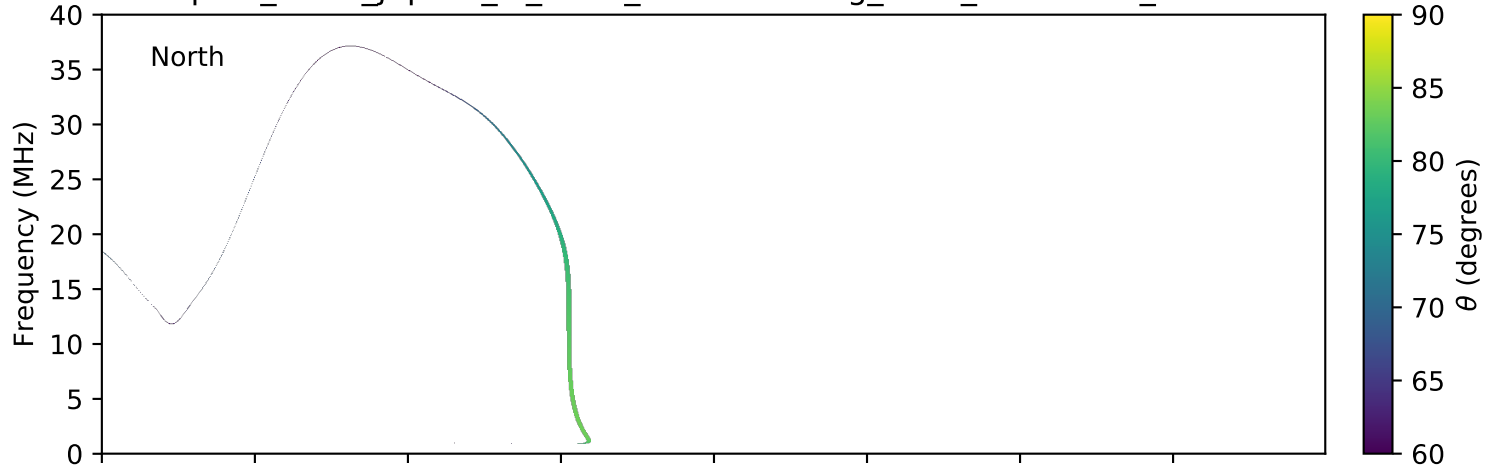
expres_earth_jupiter_io_isaac_lossc-wid1deg_3kev_20080608_v01.cdf
