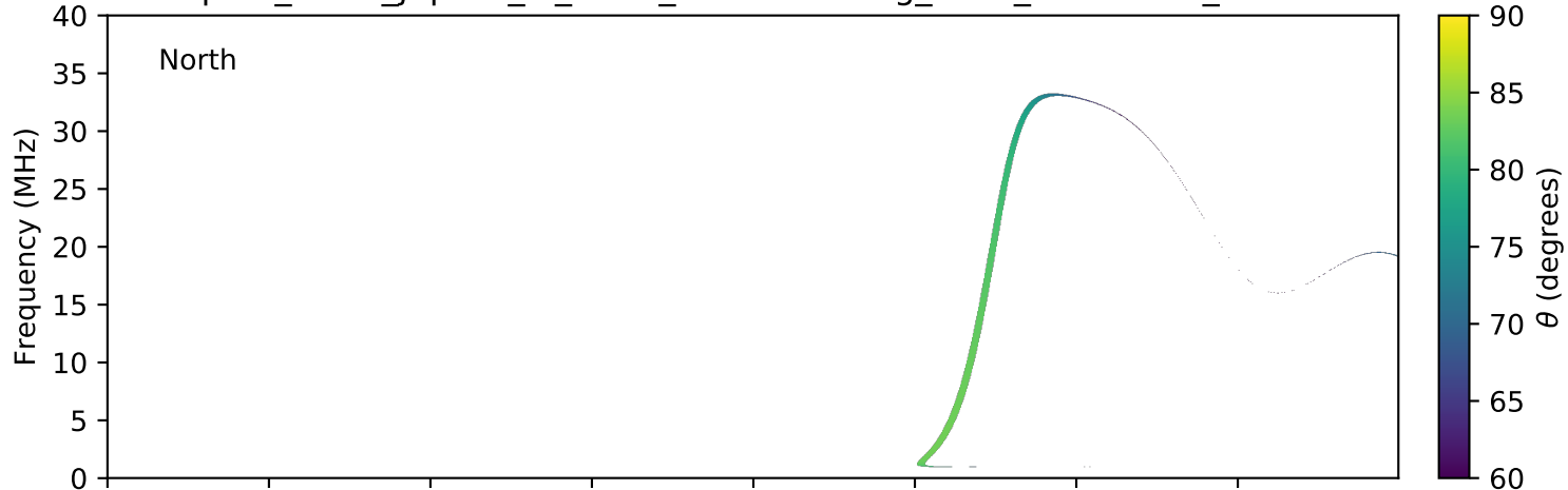
expres_earth_jupiter_io_isaac_lossc-wid1deg_3kev_20080607_v01.cdf
