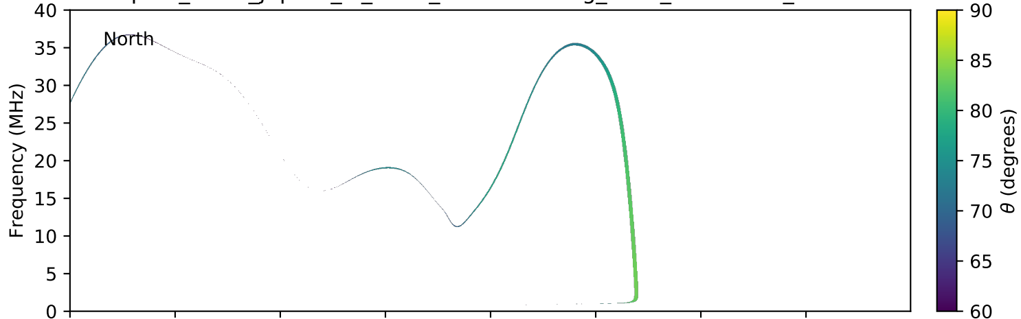
expres_earth_jupiter_io_isaac_lossc-wid1deg_3kev_20080606_v01.cdf
