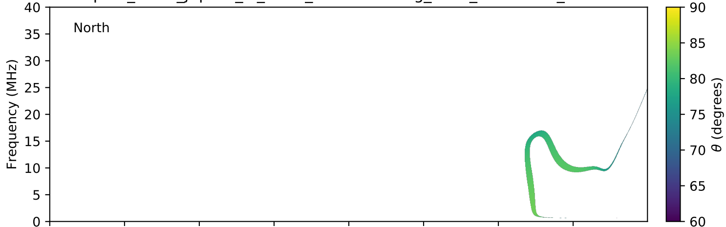
expres_earth_jupiter_io_isaac_lossc-wid1deg_3kev_20080605_v01.cdf
