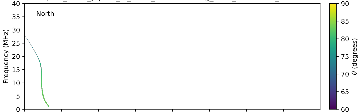
expres_earth_jupiter_io_isaac_lossc-wid1deg_3kev_20080603_v01.cdf
