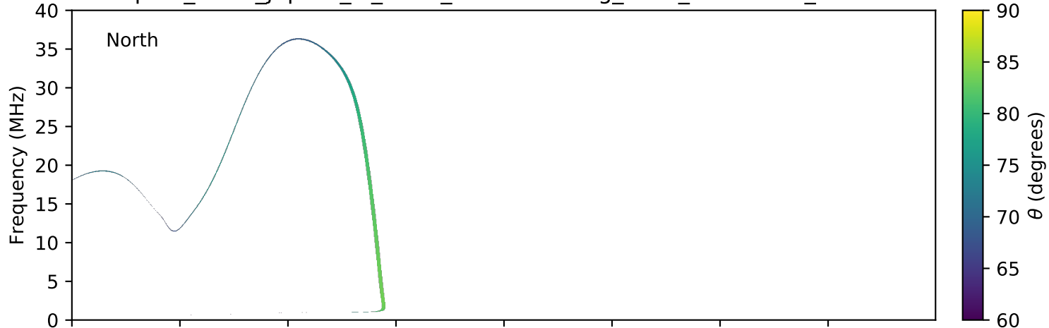
expres_earth_jupiter_io_isaac_lossc-wid1deg_3kev_20080601_v01.cdf
