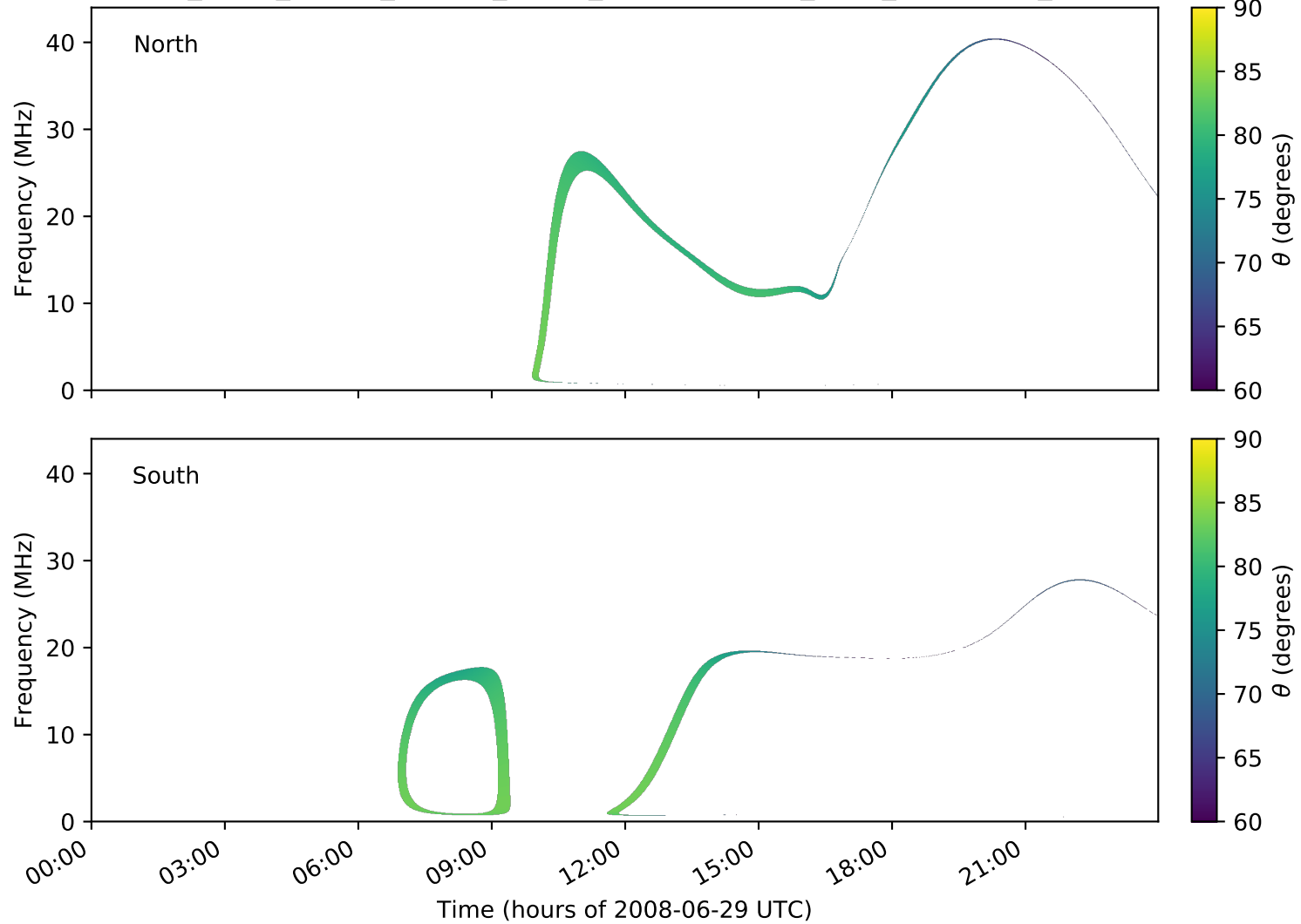
expres_earth_jupiter_europa_jrm09_lossc-wid1deg_3kev_20080629_v01.cdf
