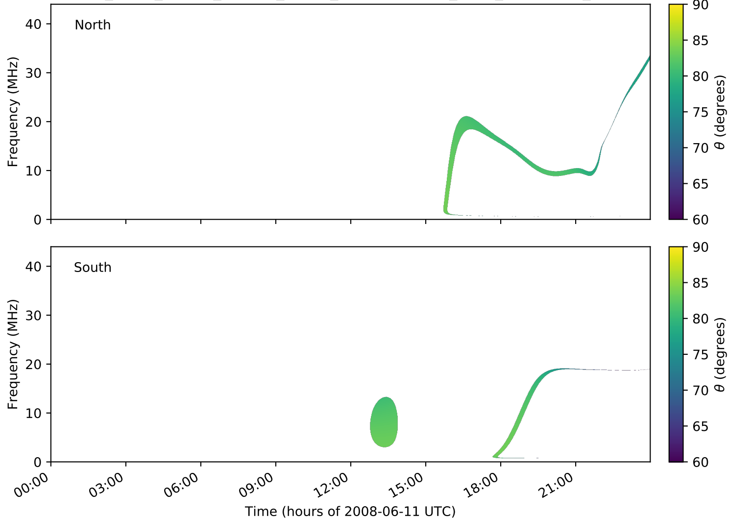
expres_earth_jupiter_europa_jrm09_lossc-wid1deg_3kev_20080611_v01.cdf
