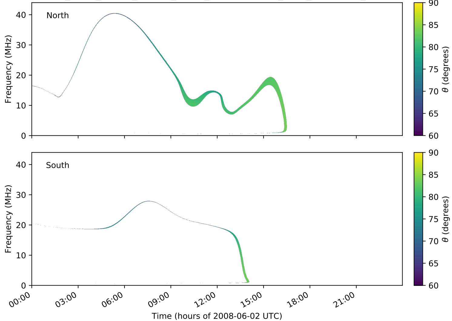
expres_earth_jupiter_europa_jrm09_lossc-wid1deg_3kev_20080602_v01.cdf
