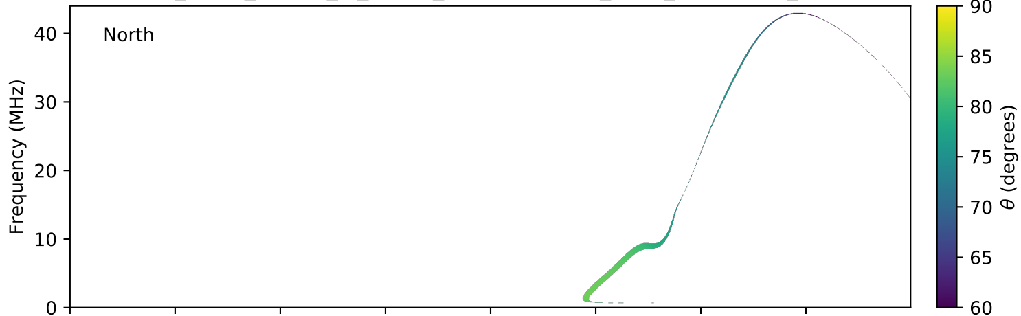
expres_earth_jupiter_io_jrm09_lossc-wid1deg_3kev_20080330_v01.cdf
