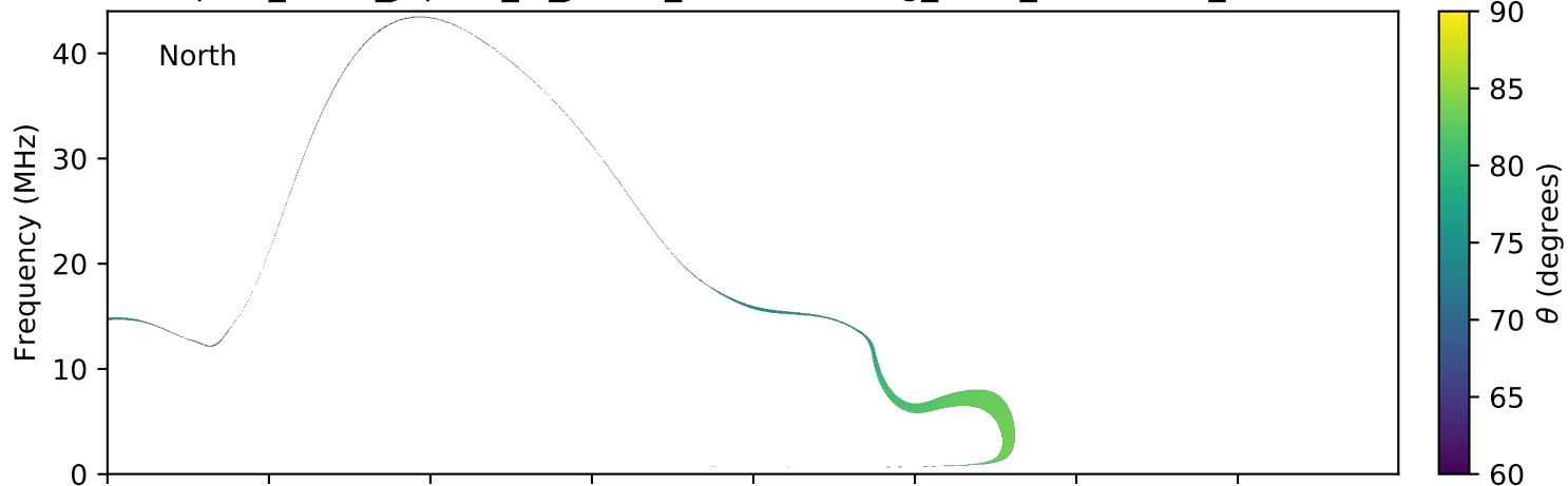
expres_earth_jupiter_io_jrm09_lossc-wid1deg_3kev_20080329_v01.cdf
