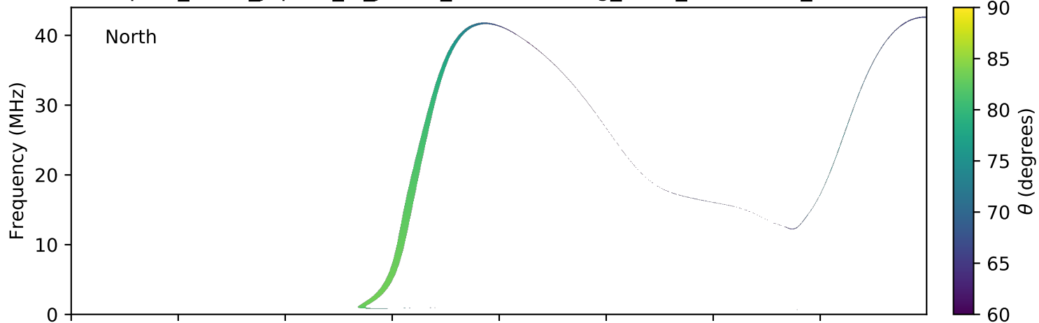
expres_earth_jupiter_io_jrm09_lossc-wid1deg_3kev_20080325_v01.cdf
