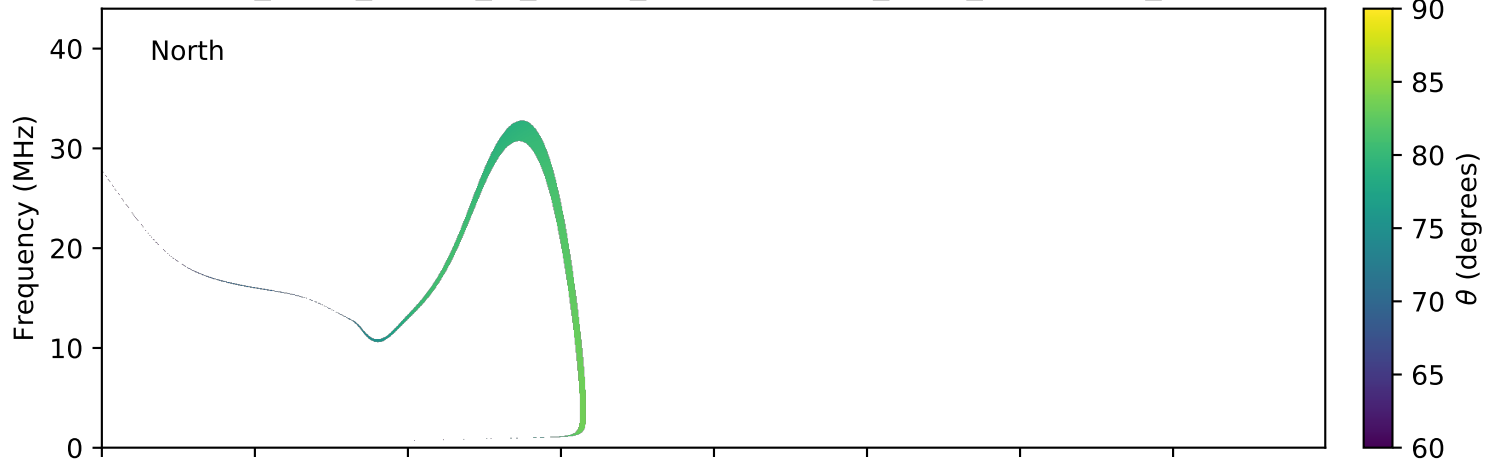
expres_earth_jupiter_io_jrm09_lossc-wid1deg_3kev_20080324_v01.cdf
