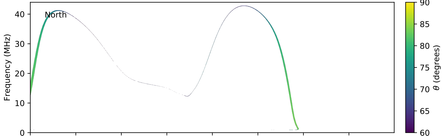
expres_earth_jupiter_io_jrm09_lossc-wid1deg_3kev_20080313_v01.cdf
