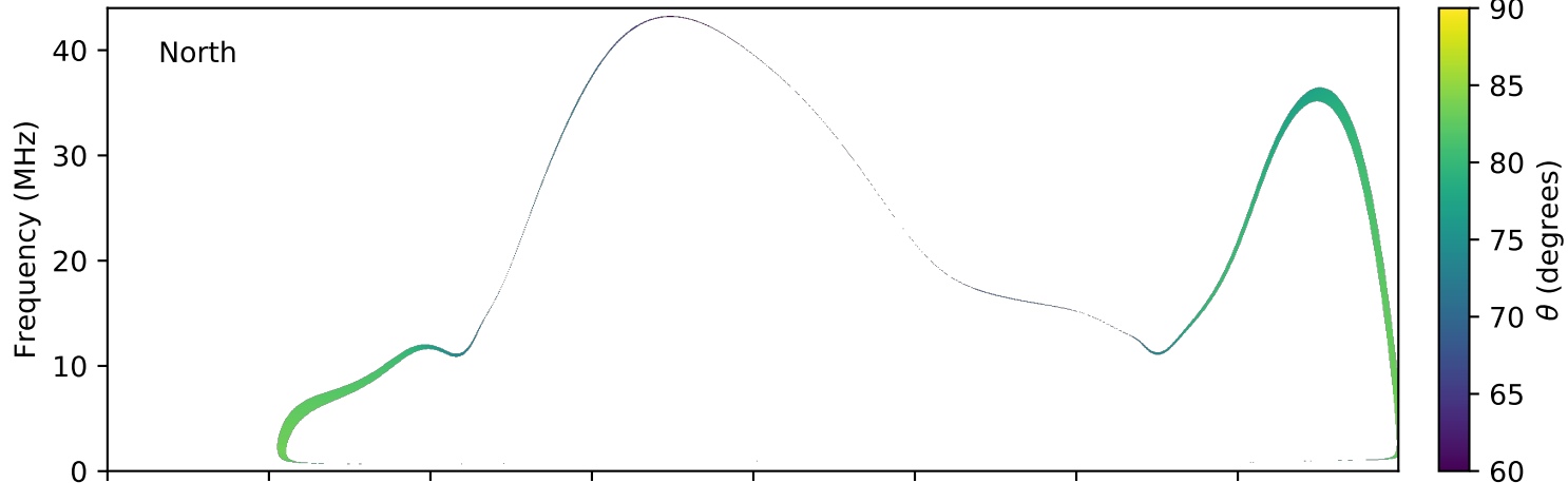
expres_earth_jupiter_io_jrm09_lossc-wid1deg_3kev_20080311_v01.cdf
