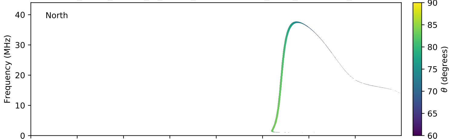
expres_earth_jupiter_io_jrm09_lossc-wid1deg_3kev_20080307_v01.cdf
