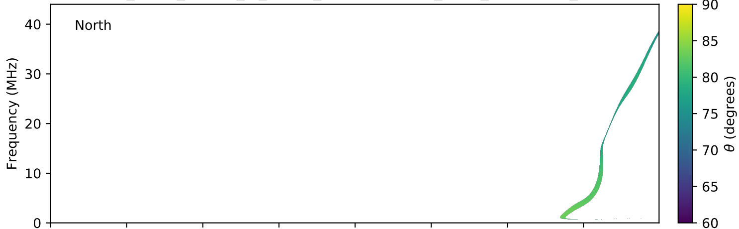
expres_earth_jupiter_io_jrm09_lossc-wid1deg_3kev_20080305_v01.cdf
