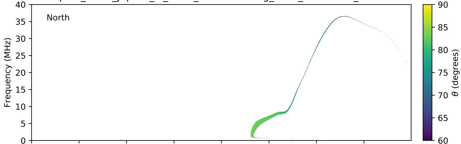
expres_earth_jupiter_io_isaac_lossc-wid1deg_3kev_20080330_v01.cdf
