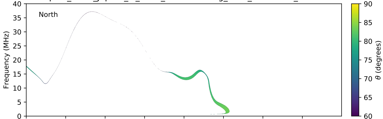
expres_earth_jupiter_io_isaac_lossc-wid1deg_3kev_20080329_v01.cdf
