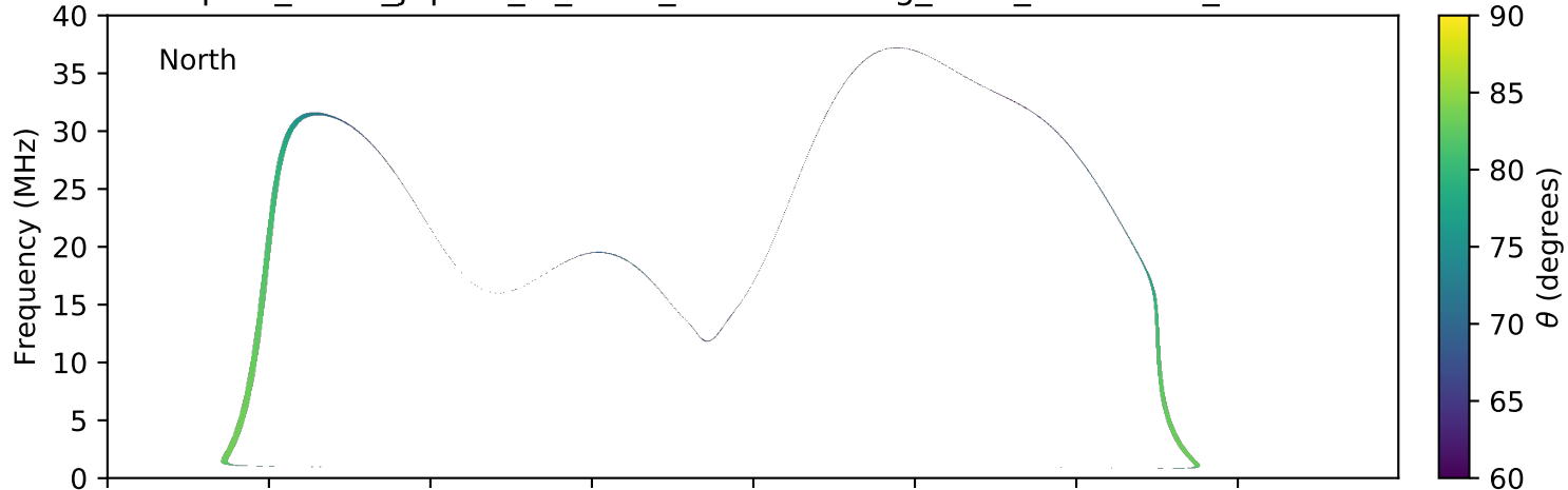
expres_earth_jupiter_io_isaac_lossc-wid1deg_3kev_20080327_v01.cdf
