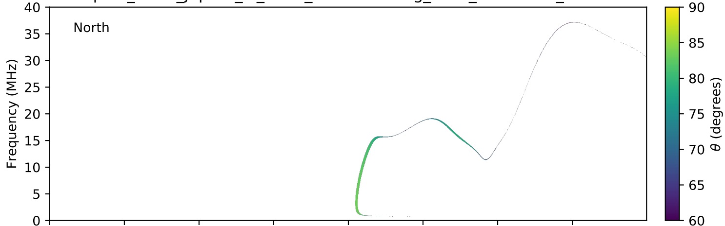
expres_earth_jupiter_io_isaac_lossc-wid1deg_3kev_20080323_v01.cdf
