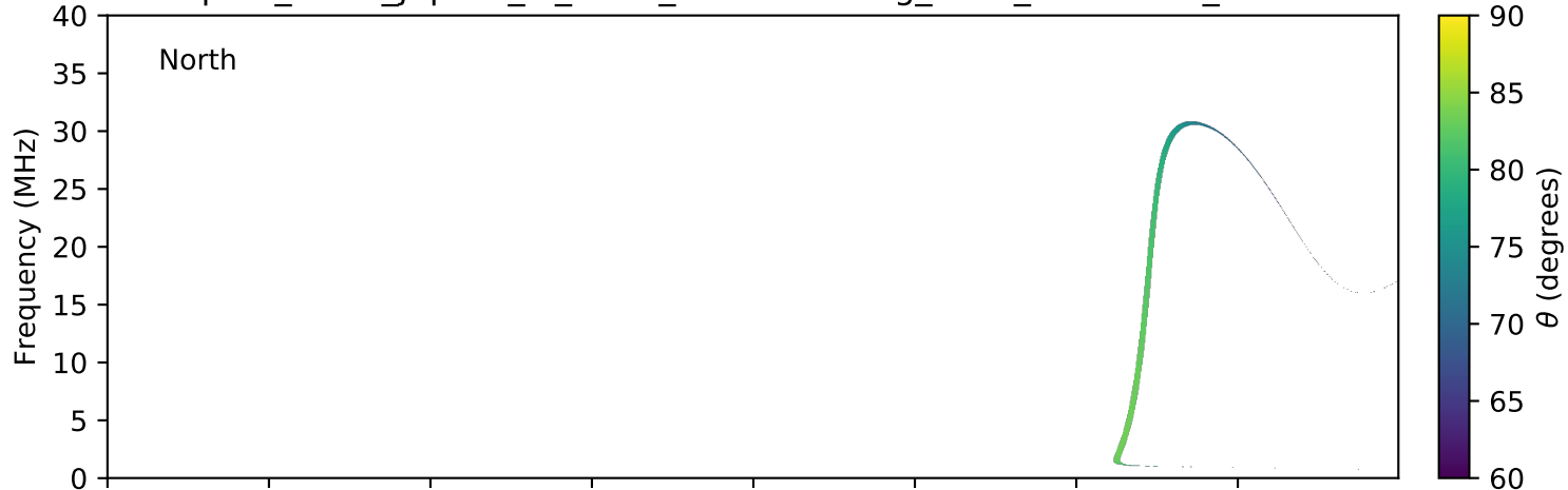
expres_earth_jupiter_io_isaac_lossc-wid1deg_3kev_20080321_v01.cdf
