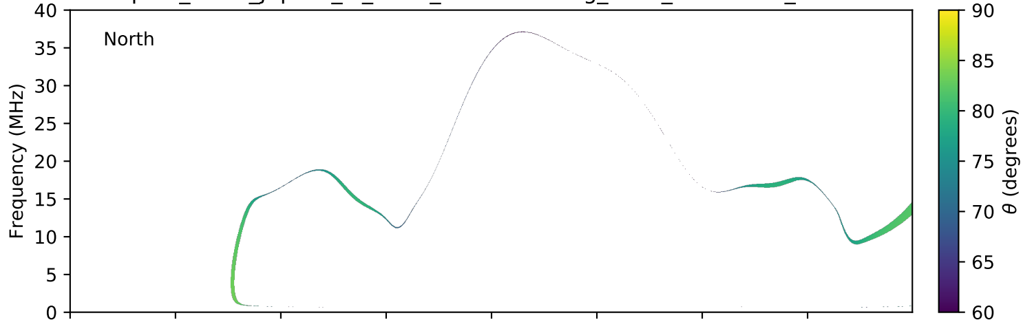
expres_earth_jupiter_io_isaac_lossc-wid1deg_3kev_20080318_v01.cdf
