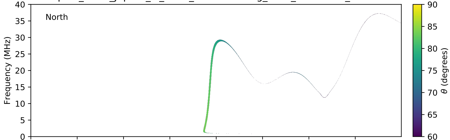
expres_earth_jupiter_io_isaac_lossc-wid1deg_3kev_20080316_v01.cdf
