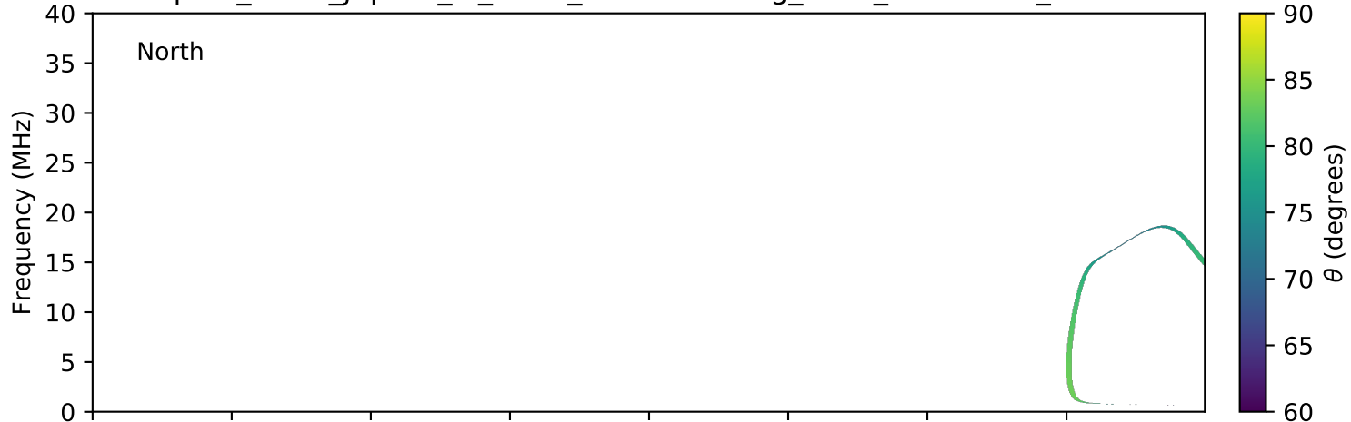
expres_earth_jupiter_io_isaac_lossc-wid1deg_3kev_20080312_v01.cdf
