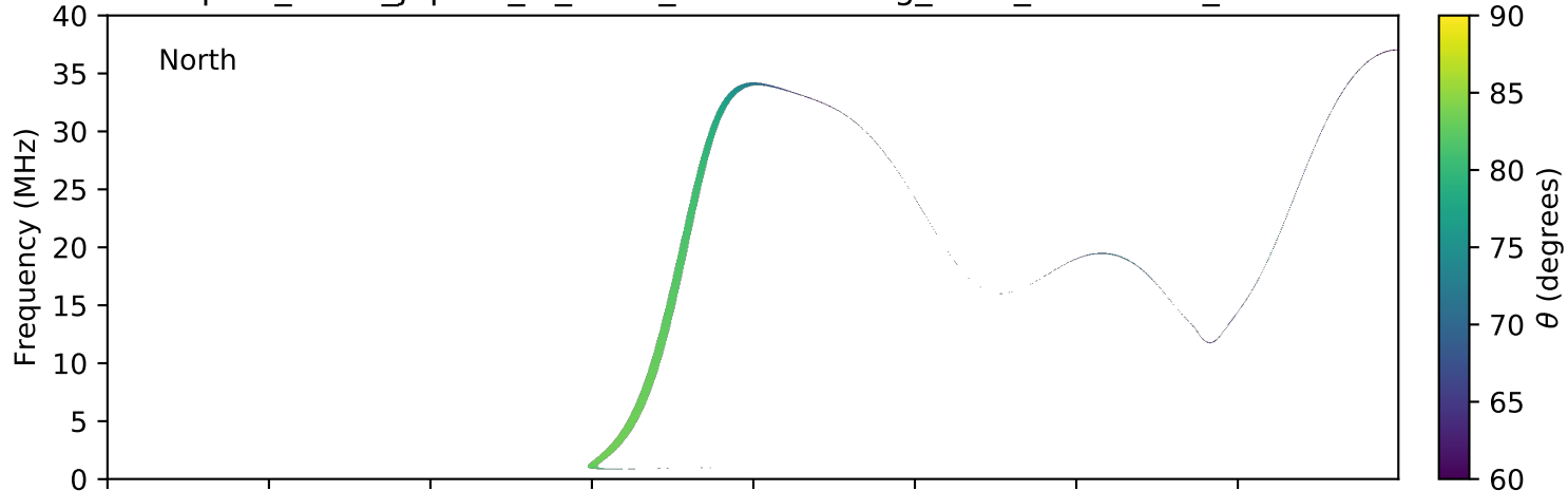
expres_earth_jupiter_io_isaac_lossc-wid1deg_3kev_20080309_v01.cdf
