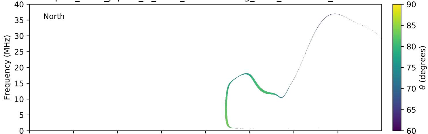
expres_earth_jupiter_io_isaac_lossc-wid1deg_3kev_20080307_v01.cdf
