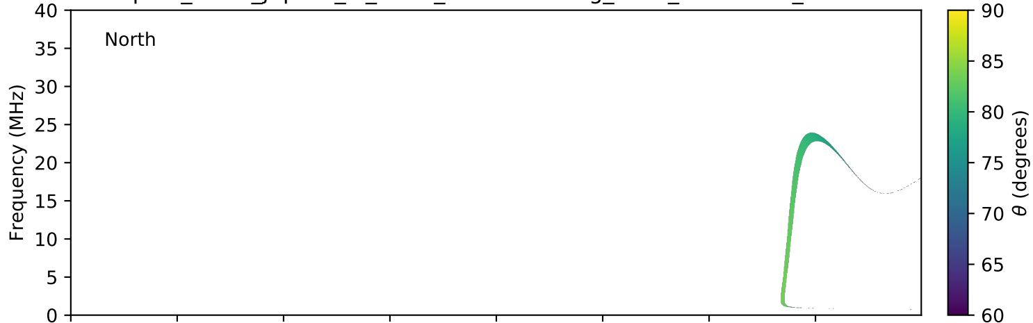
expres_earth_jupiter_io_isaac_lossc-wid1deg_3kev_20080305_v01.cdf
