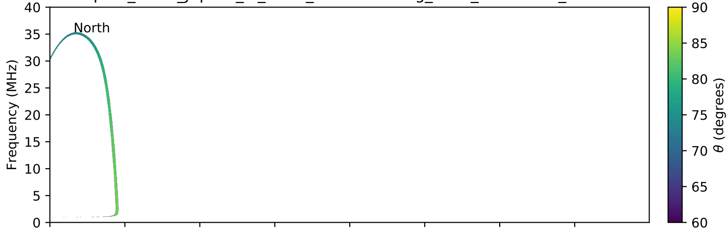
expres_earth_jupiter_io_isaac_lossc-wid1deg_3kev_20080303_v01.cdf
