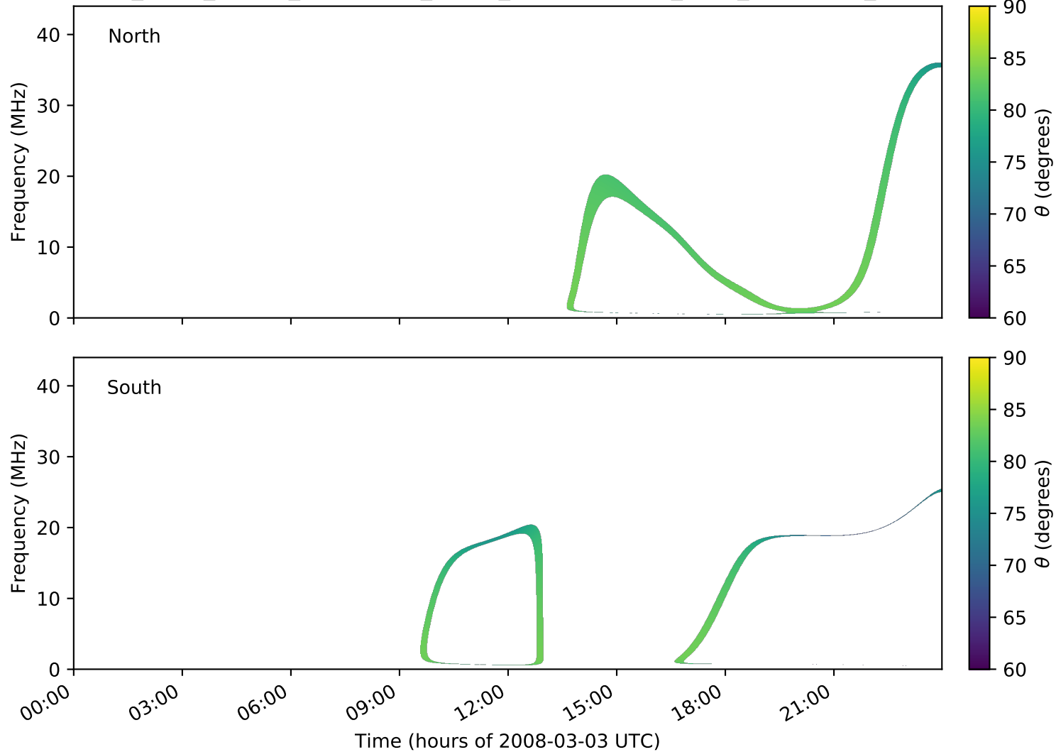
expres_earth_jupiter_ganymede_jrm09_lossc-wid1deg_3kev_20080303_v01.cdf
