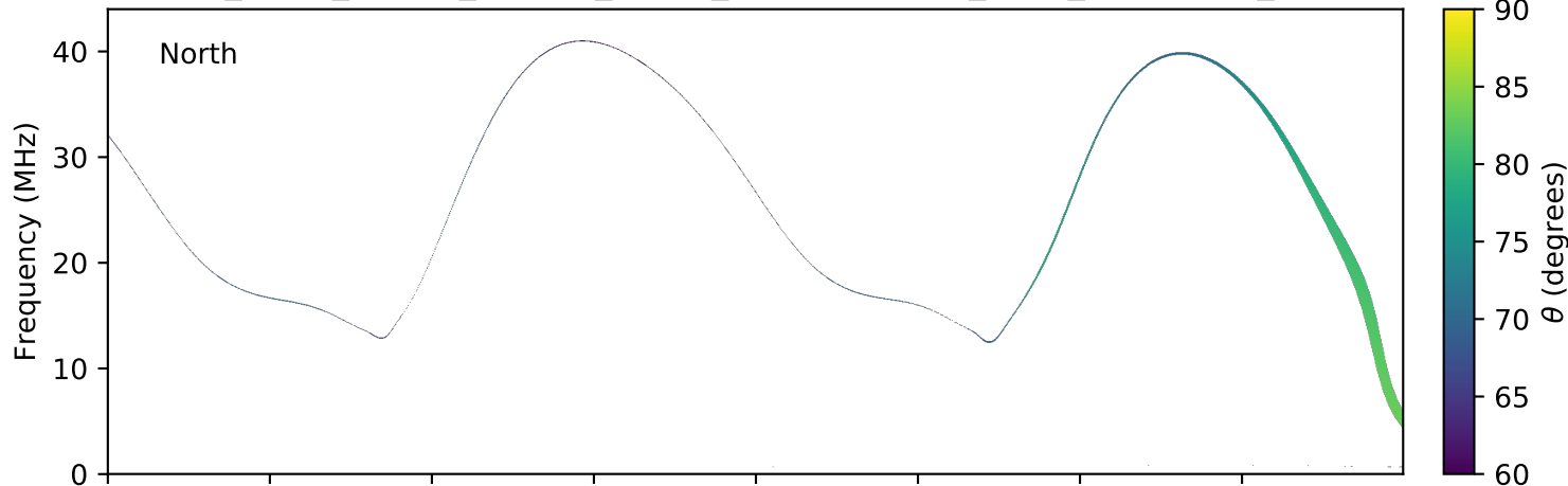
expres_earth_jupiter_europa_jrm09_lossc-wid1deg_3kev_20080326_v01.cdf
