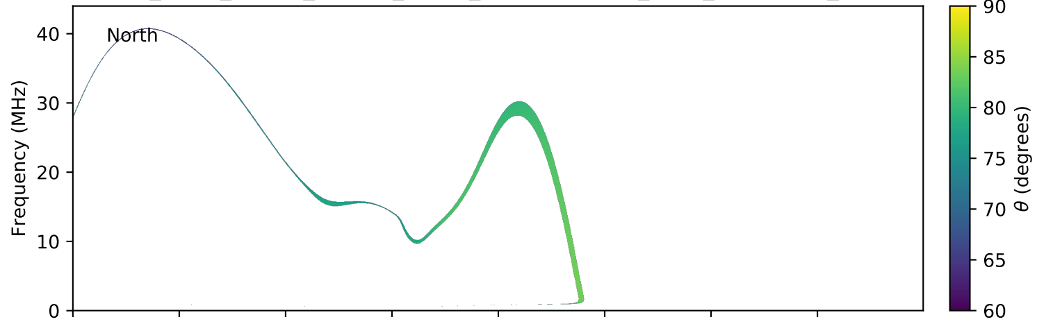
expres_earth_jupiter_europa_jrm09_lossc-wid1deg_3kev_20080323_v01.cdf
