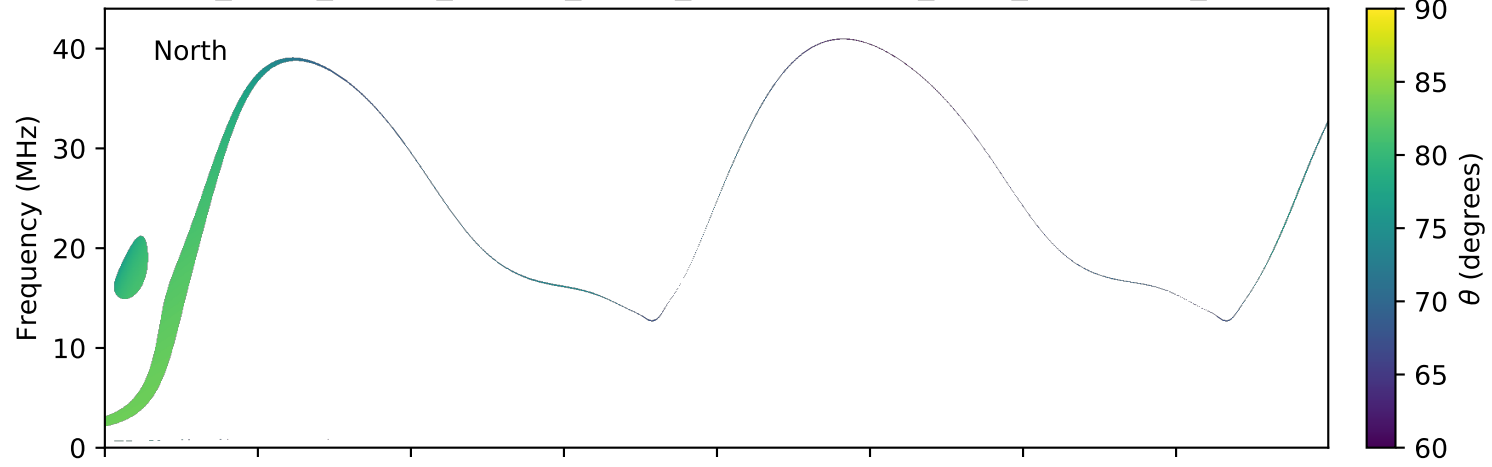
expres_earth_jupiter_europa_jrm09_lossc-wid1deg_3kev_20080315_v01.cdf
