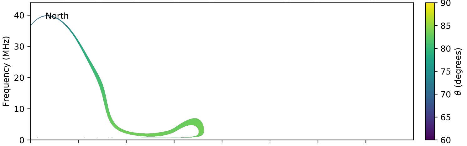
expres_earth_jupiter_europa_jrm09_lossc-wid1deg_3kev_20080309_v01.cdf
