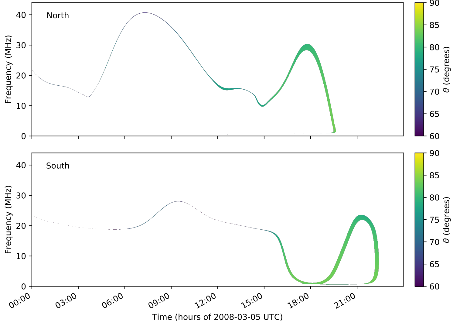
expres_earth_jupiter_europa_jrm09_lossc-wid1deg_3kev_20080305_v01.cdf
