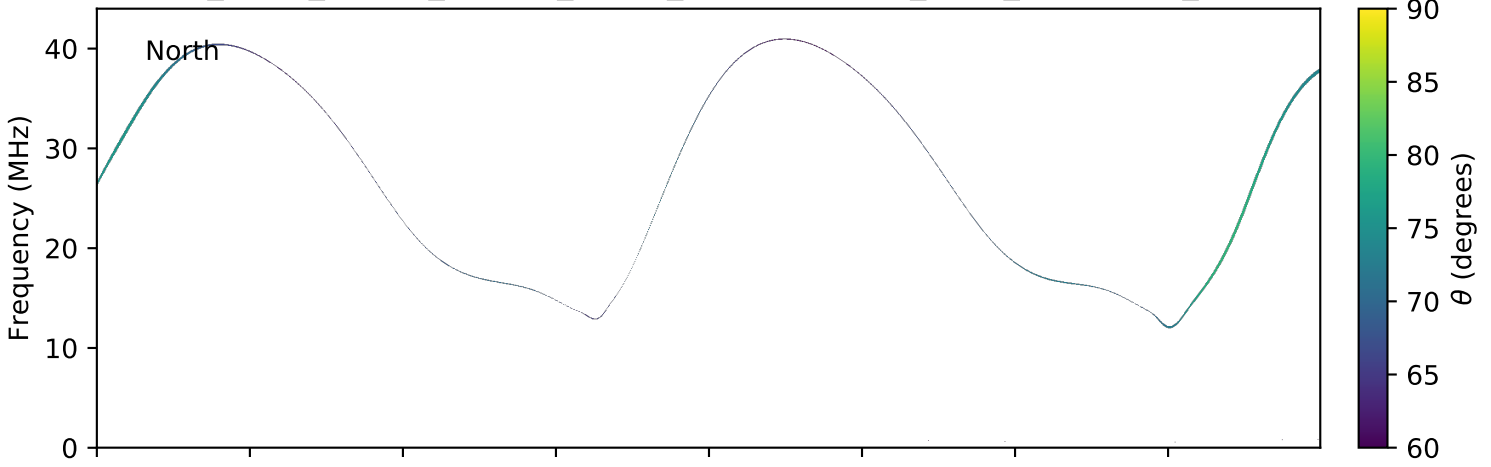
expres_earth_jupiter_europa_jrm09_lossc-wid1deg_3kev_20080301_v01.cdf
