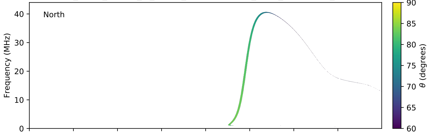
expres_earth_jupiter_io_jrm09_lossc-wid1deg_3kev_20080229_v01.cdf
