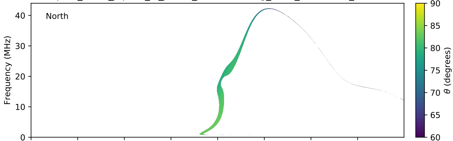
expres_earth_jupiter_io_jrm09_lossc-wid1deg_3kev_20080222_v01.cdf
