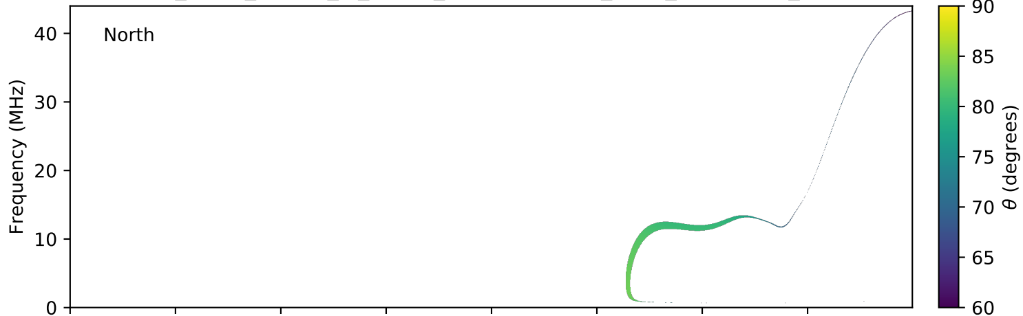
expres_earth_jupiter_io_jrm09_lossc-wid1deg_3kev_20080220_v01.cdf
