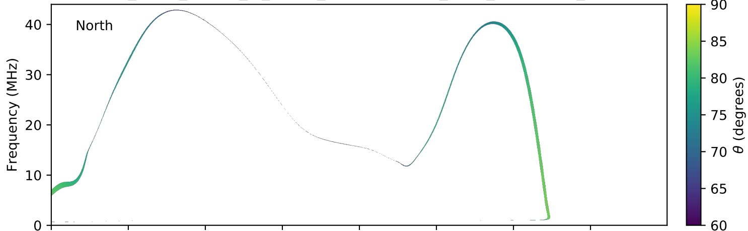
expres_earth_jupiter_io_jrm09_lossc-wid1deg_3kev_20080203_v01.cdf
